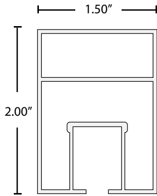
Rail Dimensions
