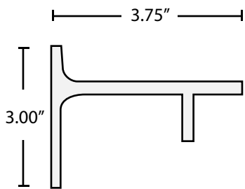
Bracket Dimensions
