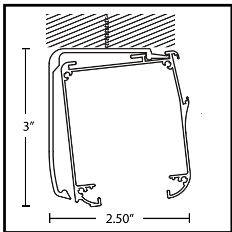
Ceiling Mount
