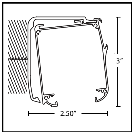
Wall Mount
