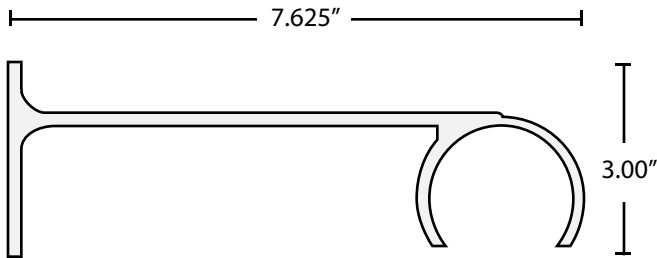
Bracket Dimensions
