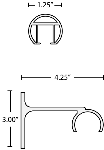
Rail Dimensions
